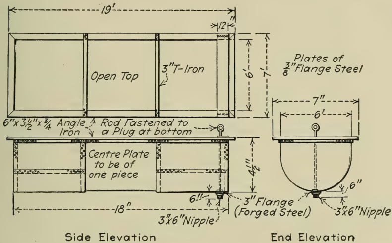
FIG. 25.—Steel Melting Tank.
